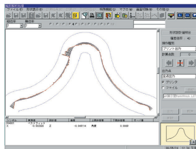
Contour profile nominal value collation
